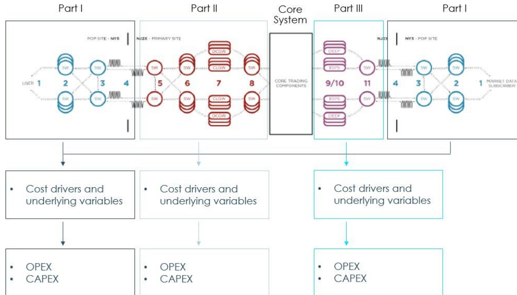
Figure 8 The physical infrastructure that comprises the Core Trading System of the IEX
